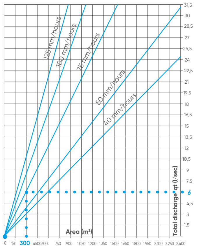
Picture 3 Flow rate calculation
