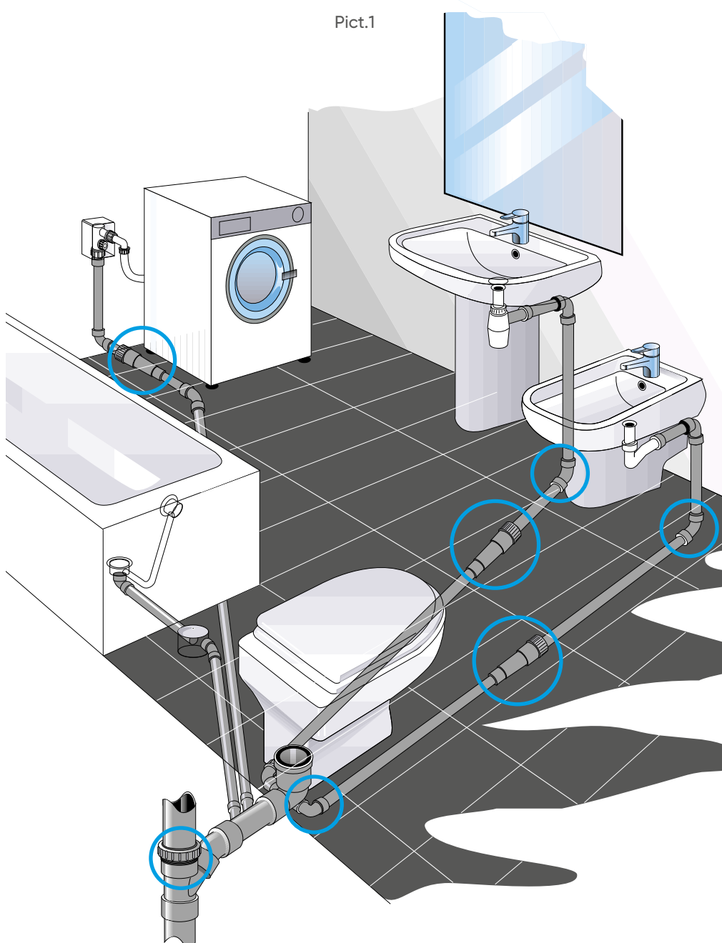
Expansion joint horizontal •A •B •C
