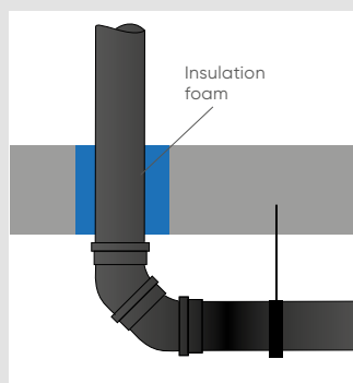
Passage through the floor. (Up to 10 m pipe drop).
