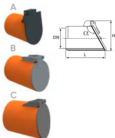
Type A INOX FLAP
