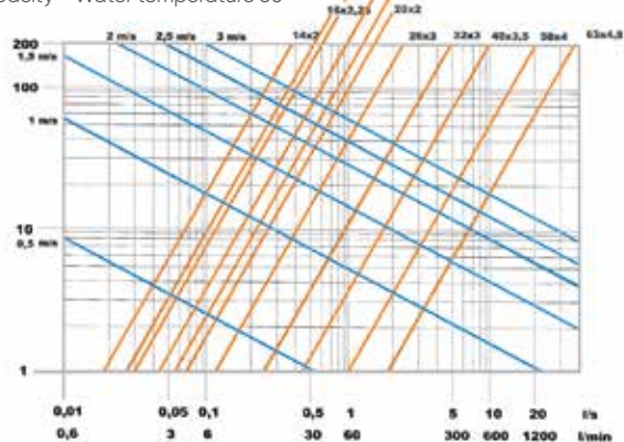
Load loss diagram - \Delta L (MBAR/M)
