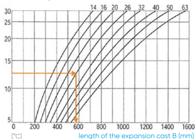
Expansion length \Delta L (mm)
