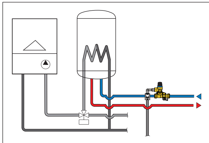
Application diagram 528 series
