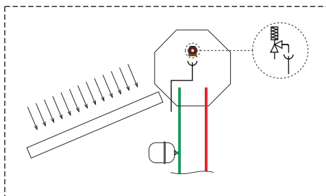
Application diagram of thermostatic diverter valve 2620 series
