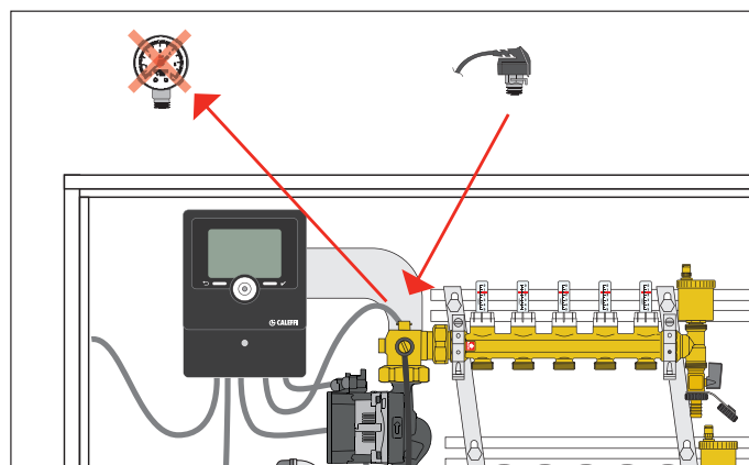
Application diagram with code 161005
