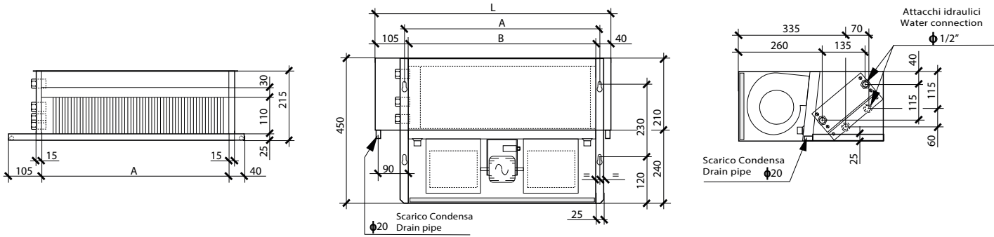
Dimensions horizontal versions
