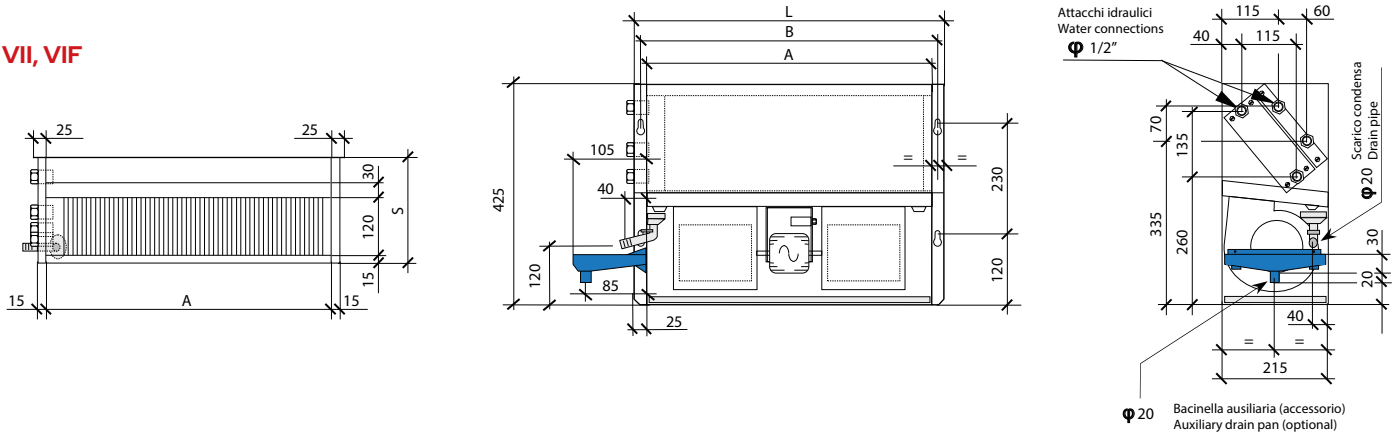
Dimensions vertical versions
